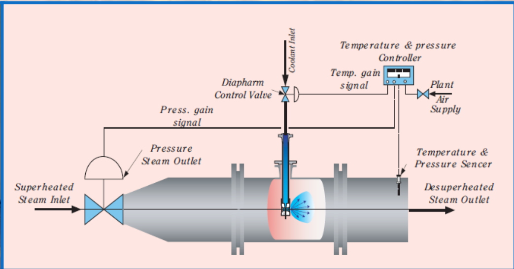
De-Super Heater
