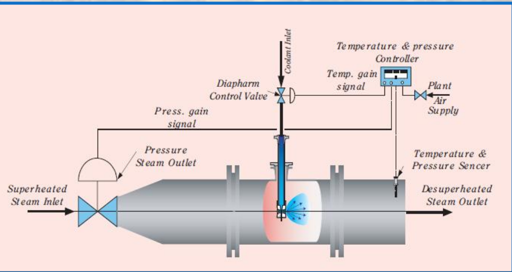
De-Super Heater
